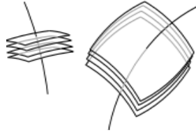
Fig(3). The 1+3 split illustrated. A field of observers with 4-velocities fills space time. At any point, space time is split into space (a hyper surface orthogonal to u^\mu ) and time (parallel to u^\mu ).
