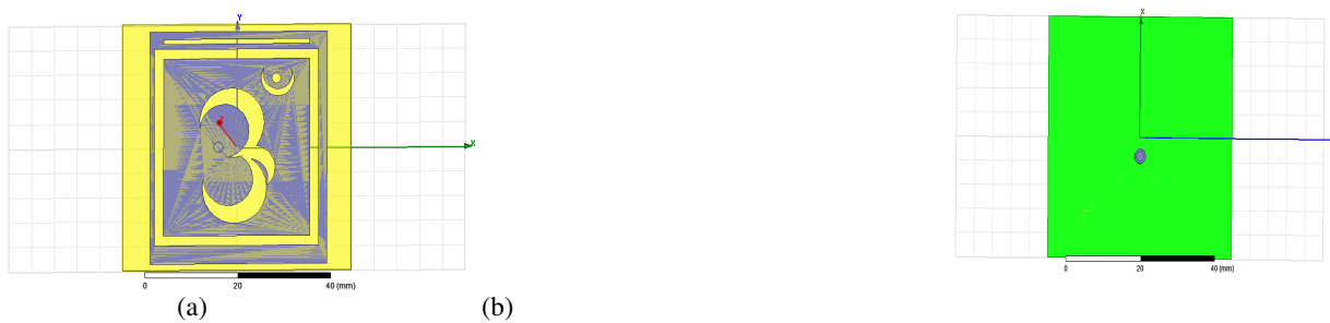
Fig 2: Microstrip patch antenna with no defected ground (a) Top view of antenna (b) bottom view of antenna
