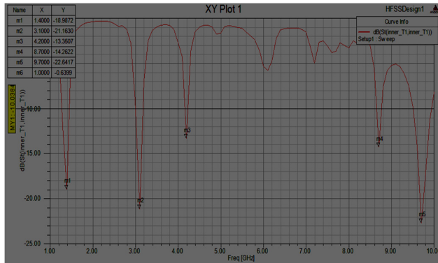
Fig 6: S11 Parameter Vs Frequency
