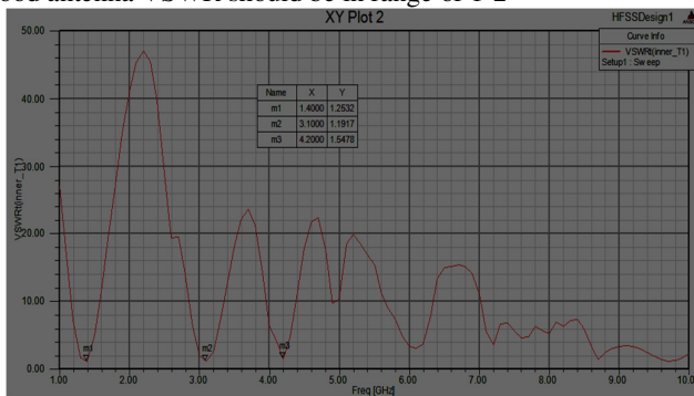
Fig 7 : VSWR Parameter for Proposed antenna
